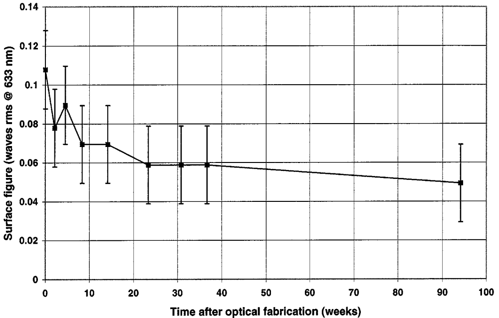
FIGURE 4.5 Temporal stability of a commercial 13-in.-diameter beryllium mirror fabricated from vacuum hot pressed block. Source: Paquin, R.A. 1992. Optomechanical Design , Yoder, P.R., ed., p. 160. CR43, SPIE Optical Engineering Press, Bellingham, WA.
