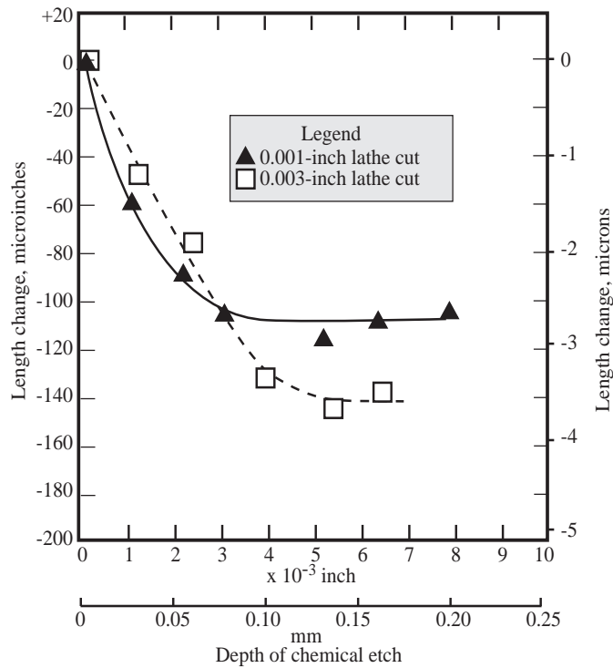
FIGURE 4.4 Dimensional changes in 3.0-in.-long specimens of Ni-Span-C on chemical removal of residual stresses due to machining.
