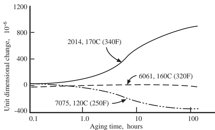
FIGURE 4.7 Dimensional change as a function of time at the precipitation heat treating temperature employed to produce the T6 temper for three aluminum alloys.
