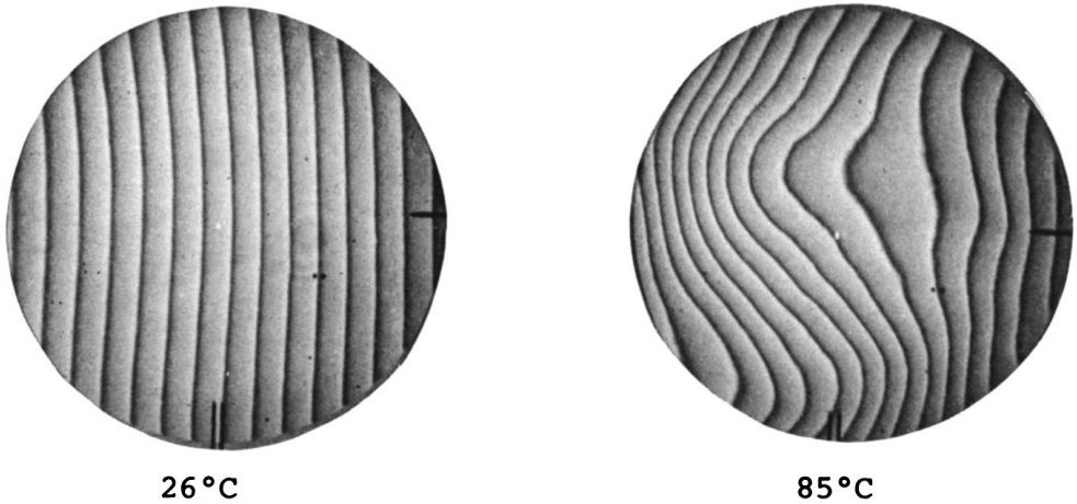
FIGURE 4.1 Optical interferograms of an electroless nickel-coated experimental beryllium alloy mirror (circa 1968) showing a reversible thermal instability of approximately two waves. Source: Paquin, R.A. 1981. Workshop on Optical Fab. and Test, Technical Digest. Optic Society of America, TB-1.
