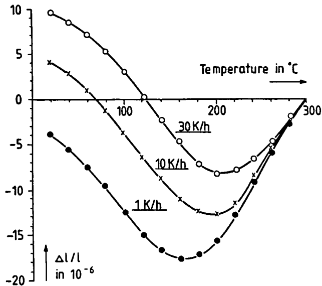
FIGURE 4.2 Thermal length contraction of Zerodur® for three cooling rates from 300 to 20°C illustrating a hysteresis type of dimensional instability. Source: Lindig, O. and Pannhorst, W. 1985. Appl. Optics , 24, 3330.
