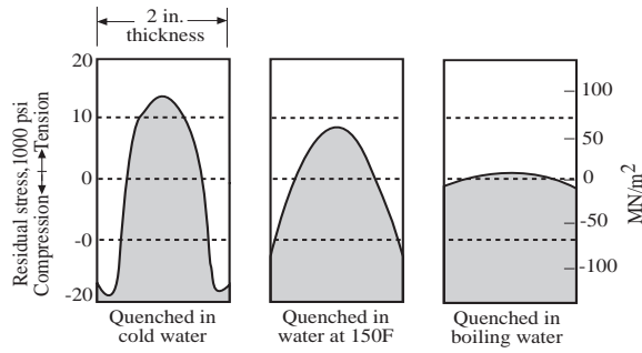
FIGURE 4.3 Residual stresses in specimens of 7075-T6 aluminum plate quenched in water at different temperatures.
