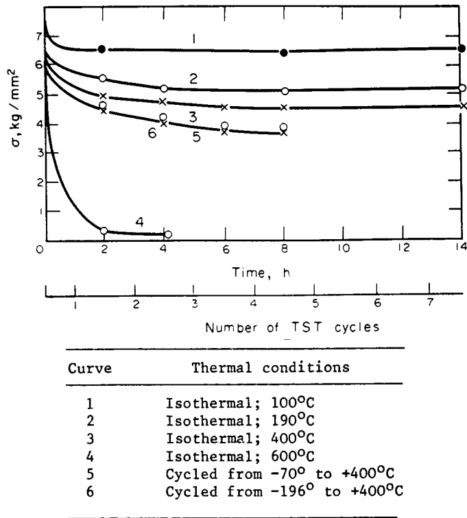
FIGURE 4.6 Comparison of the effects of thermal cycling and isothermal exposure on stress relaxation of pure beryllium. Source: Lokshin, I.Kh. 1970. Metal Sci. Heat Treat. (U.S.S.R.) , 426.
